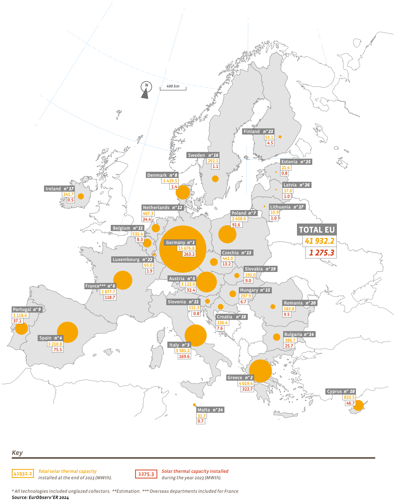
Solar thermal capacity* installed in the European Union at the end of 2023** (MWth)
